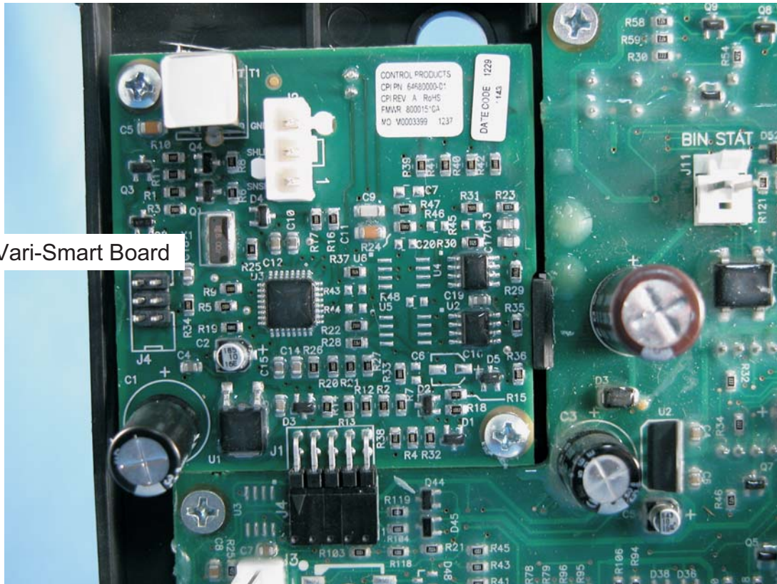
Installing Vari-Smart Board
